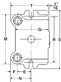
BALL BEARING
