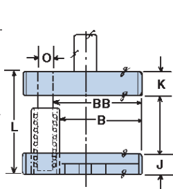
BALL BEARING
